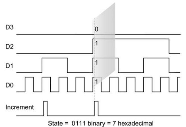
Figure 17. State acquisition captures a “slice” of data across a bus when the external clock signal enables an acquisition.
