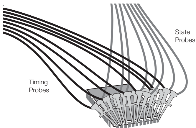
Figure 8. Double-probing requires two probes on each test point, decreasing the quality of the measurement.
