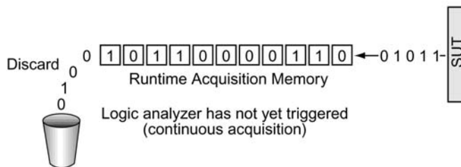
Figure 11. The logic analyzer captures and discards data on a first-in, first-out basis until a trigger event occurs.
